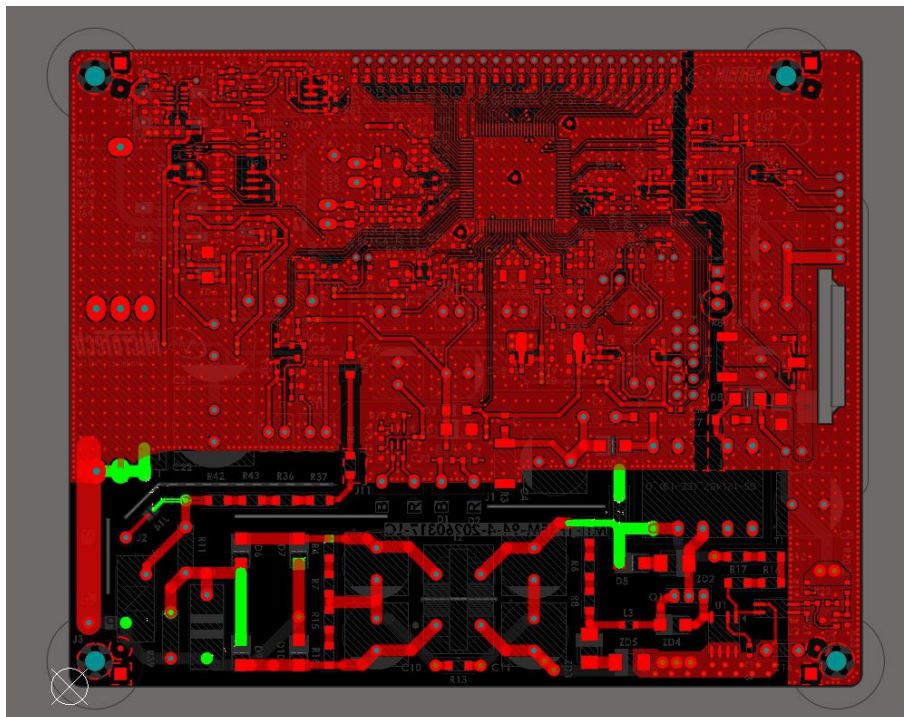
Screen Shot of the Panel PCB
